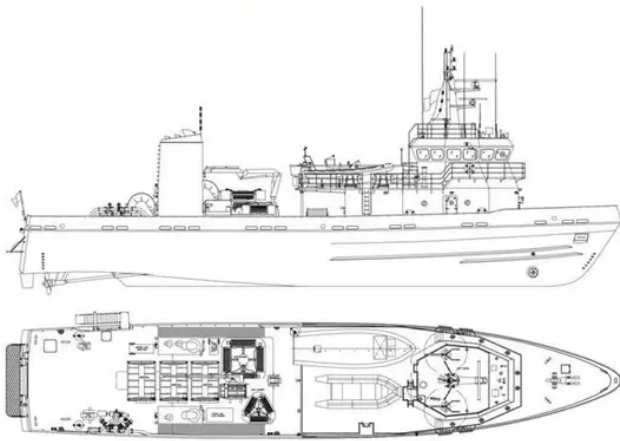
41.85m. MULTI PURPOSE VESSEL
